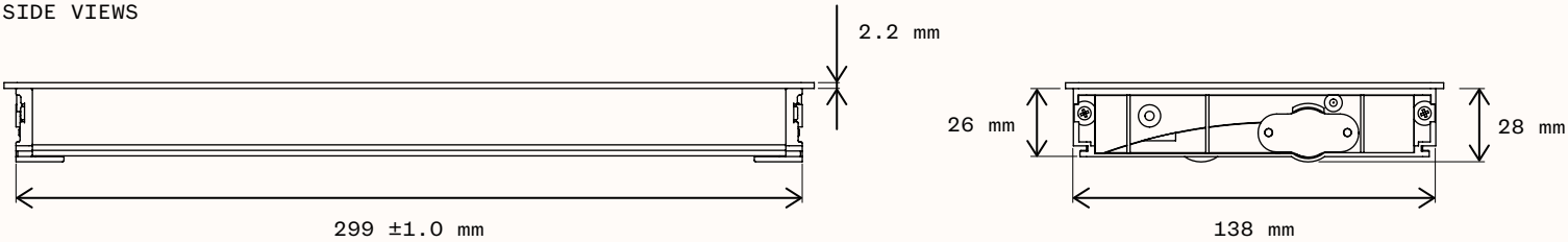
SIDE VIEWS
