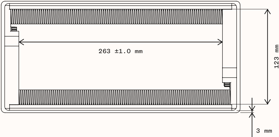
BOTTOM VIEW
